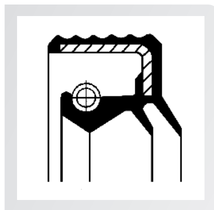
New seal with X6 (double SL dust lip) New Corteco No: 82036969
