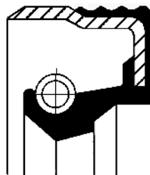
Figure 2: Oil Seal 01033415B New design - BD
