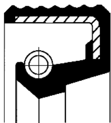
Figure 1: Oil Seal 01033415B Old design - BA
