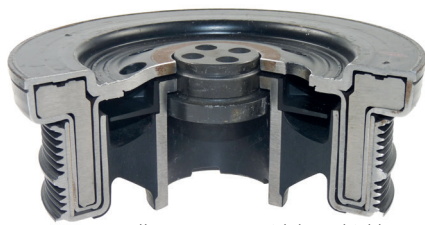
Corteco pulley 80001103 with heatshield
