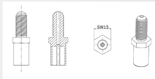
Figure 2: Joint SW15
