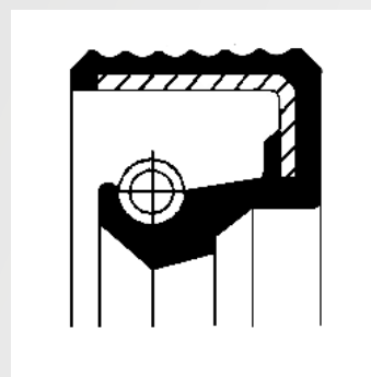
Figure 2: oil seal 12010784B new design
