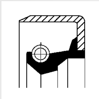
Figure 1: oil seal 01002369B old design
